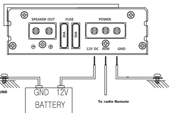
PN1.450D PN1.650D Power connection
